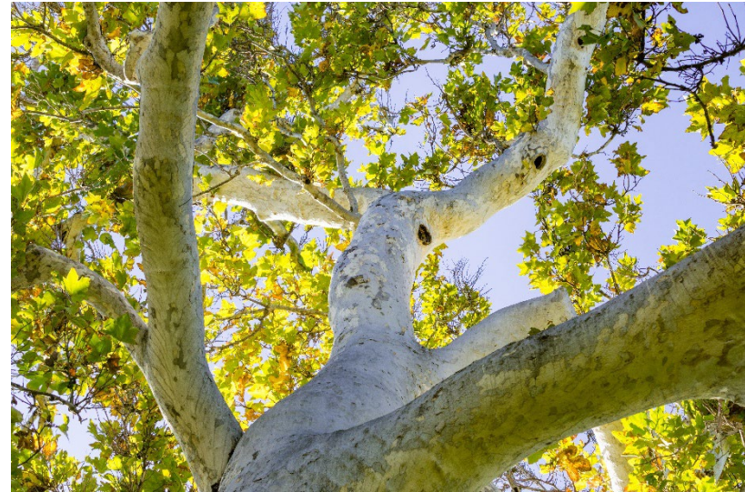
California Sycamore
